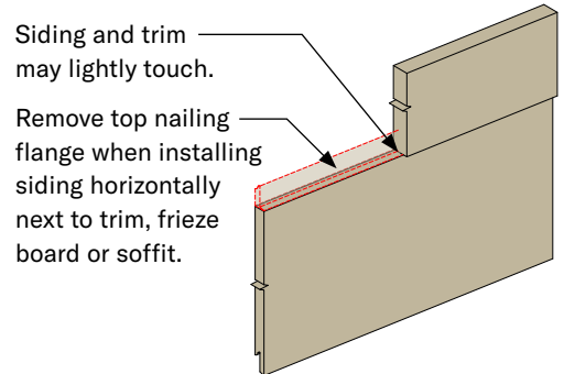
SIDING INSTALLED HORIZONTALLY Figure 9c
