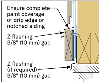
Z-FLASHING OVER DOOR & WINDOW OPENINGS PREFERRED Figure 9a
