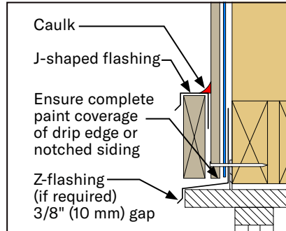
J-SHAPED FLASHING OVER DOOR & WINDOW OPENINGS ALTERNATE Figure 9b
